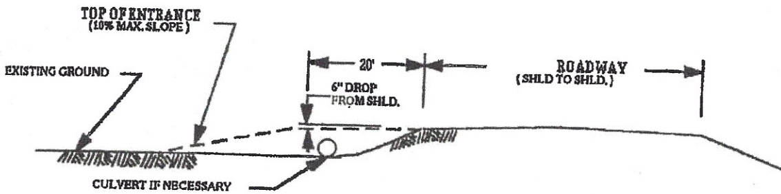
ENTRANCE WITH NO ROAD DITCH
