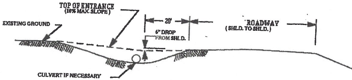
ENTRANCE ACROSS ROAD DITCH
